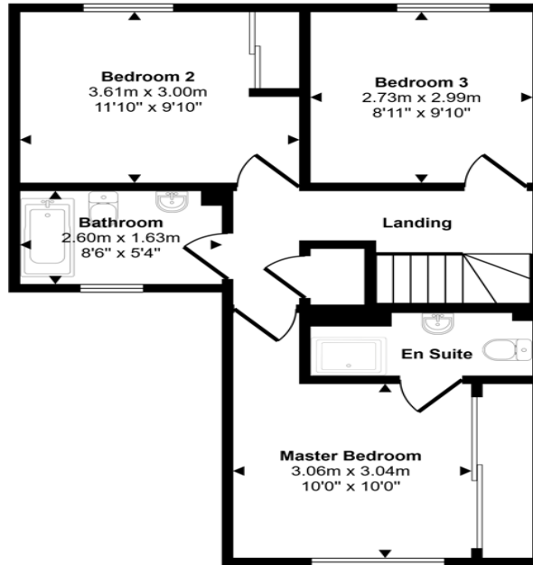
First Floor Approx 49 sq m / 531 sq ft
